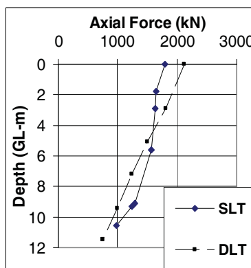
FIG. 8. Axial force distributions
