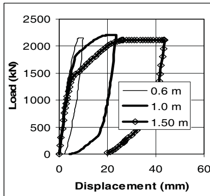
FIG. 7. CAPWAP Load-displacement curves
