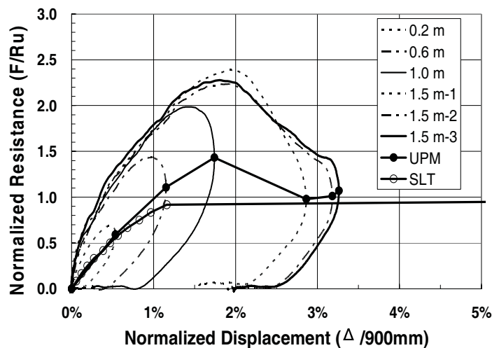
FIG. 5. Rsoil-displacement curve
